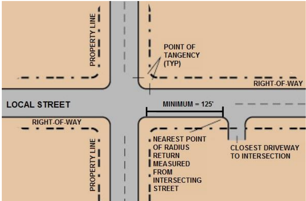
Figure 2.3 (13) Local Street Driveway Intersection Clearance
